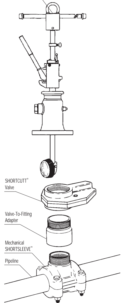
Plugging Machine
